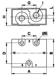
1 3/2 NC-NO G1/8 - G1/4
