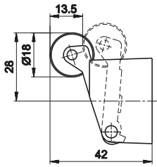
B G1/8 UNI-DIRECTIONAL ROLLER LEVER
