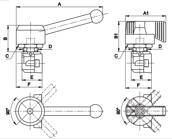
D G1/8 - G1/4 ROTATING LEVER
