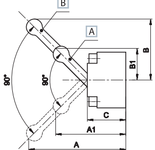
G1/8 - G1/4 SELECTOR
